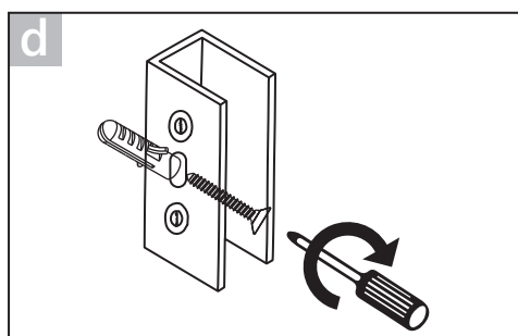
d Fasten the wall brackets with ST4*30 screws.
